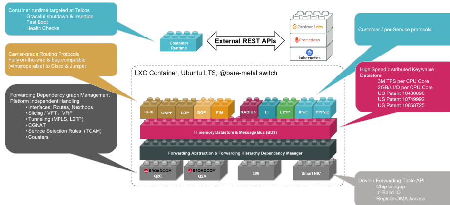
Figure 1. RBFS Overview
