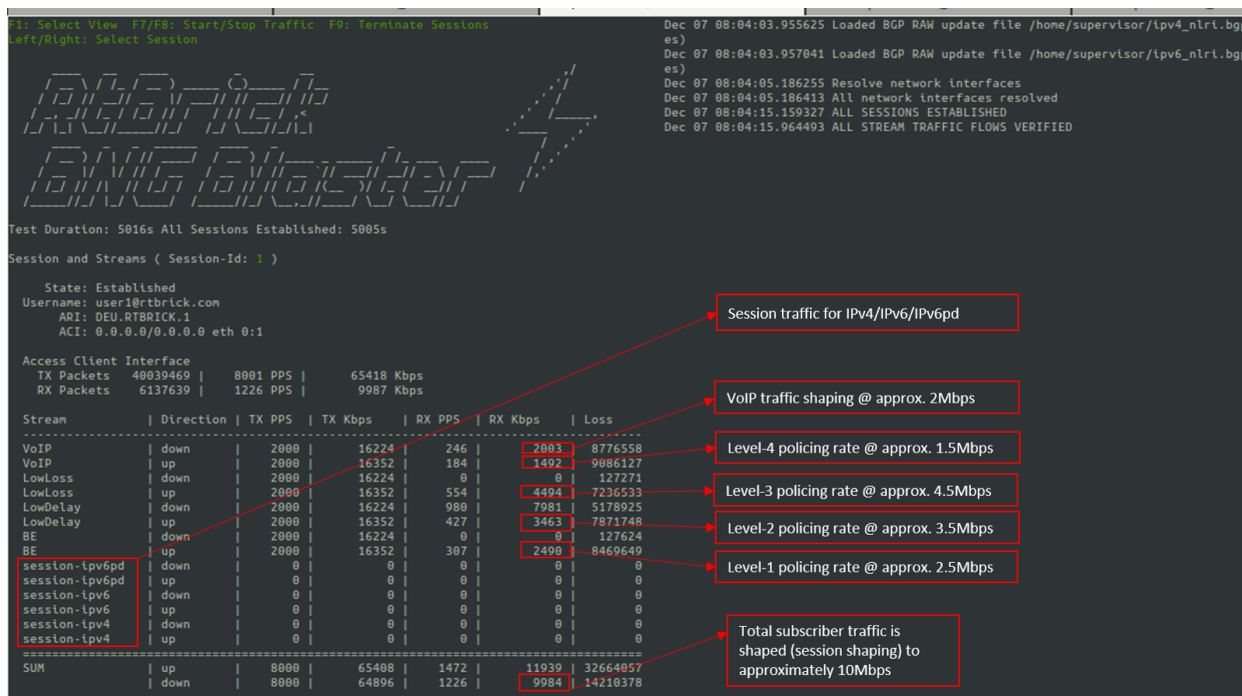
Fig 4: Reading output from BNG Blaster
