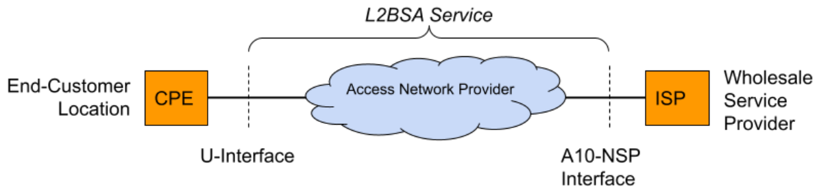
Figure 22. L2BSA Interfaces
