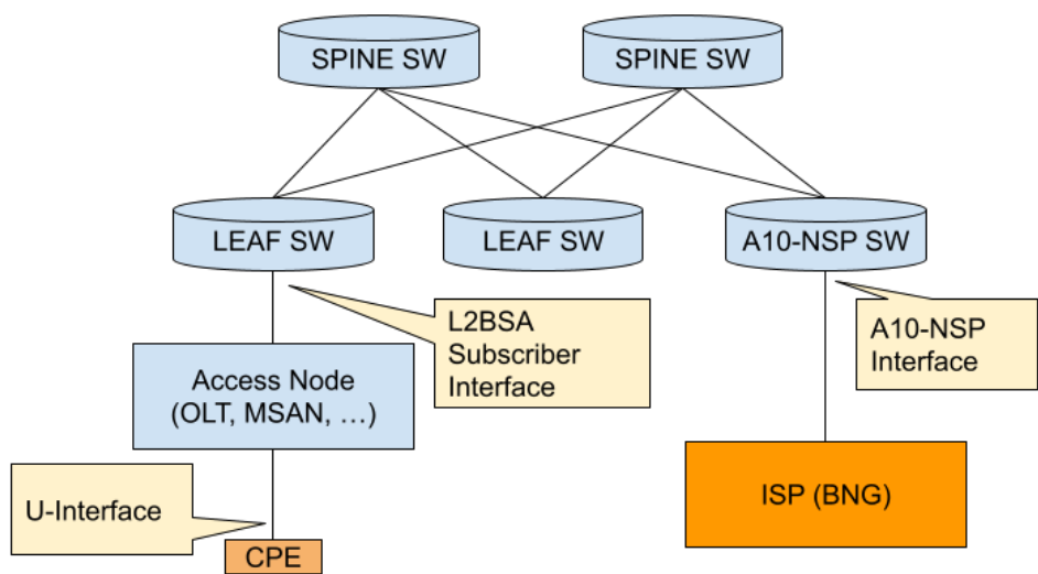
Figure 24. L2BSA Fabric
