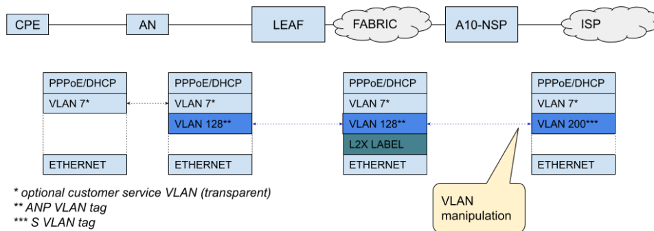
Figure 25. L2BSA Traffic
