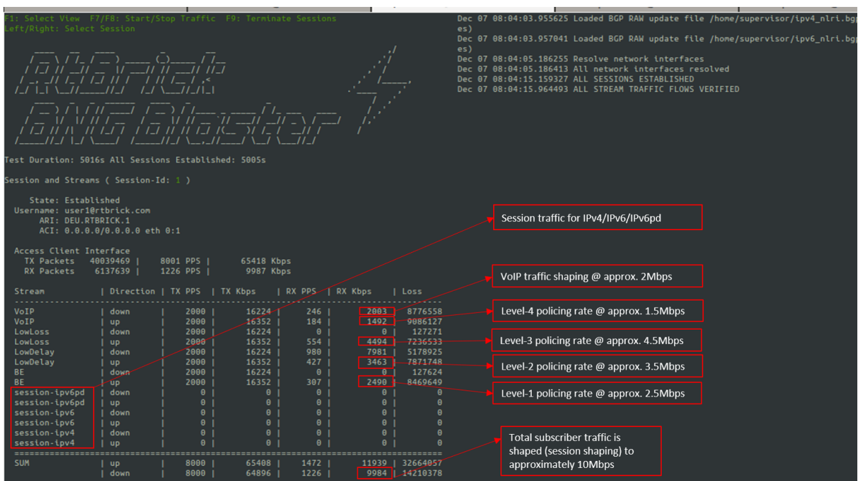
Figure 18. Reading output from BNG Blaster
