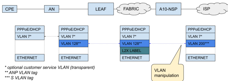
Figure 25. L2BSA Traffic
