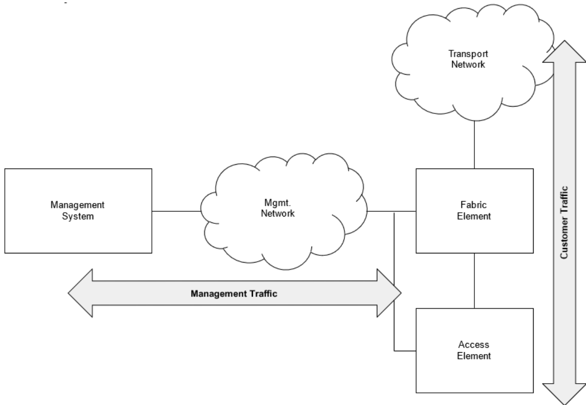
Figure 9. Schematic illustration of the out-of-band management pattern
