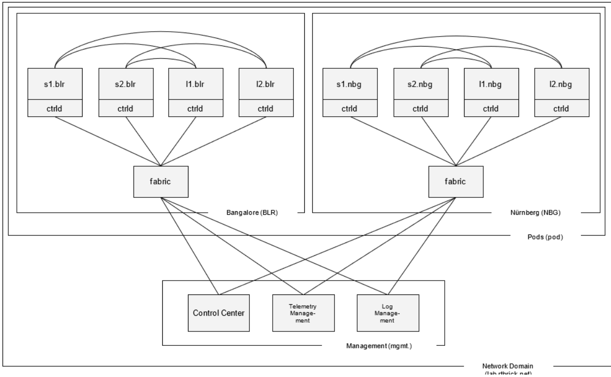
Figure 15. Sample network topology
