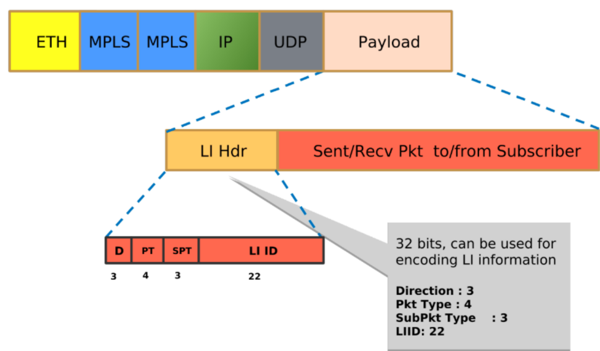
Figure 21. Packet Format Encoding
