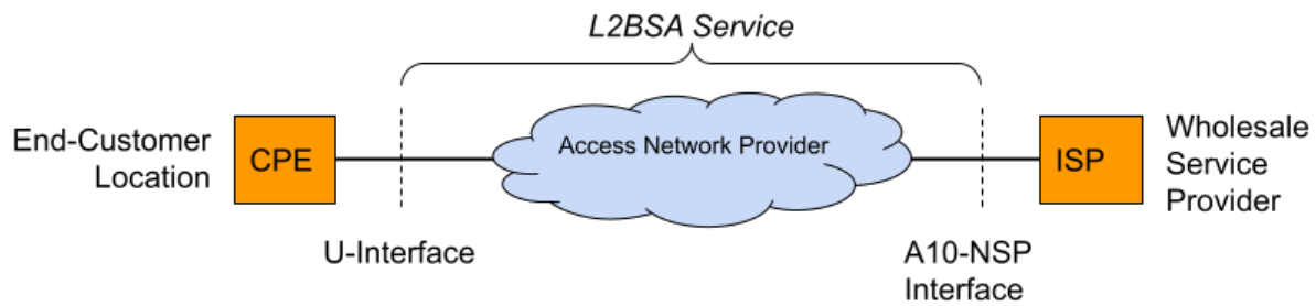
Figure 22. L2BSA Interfaces
