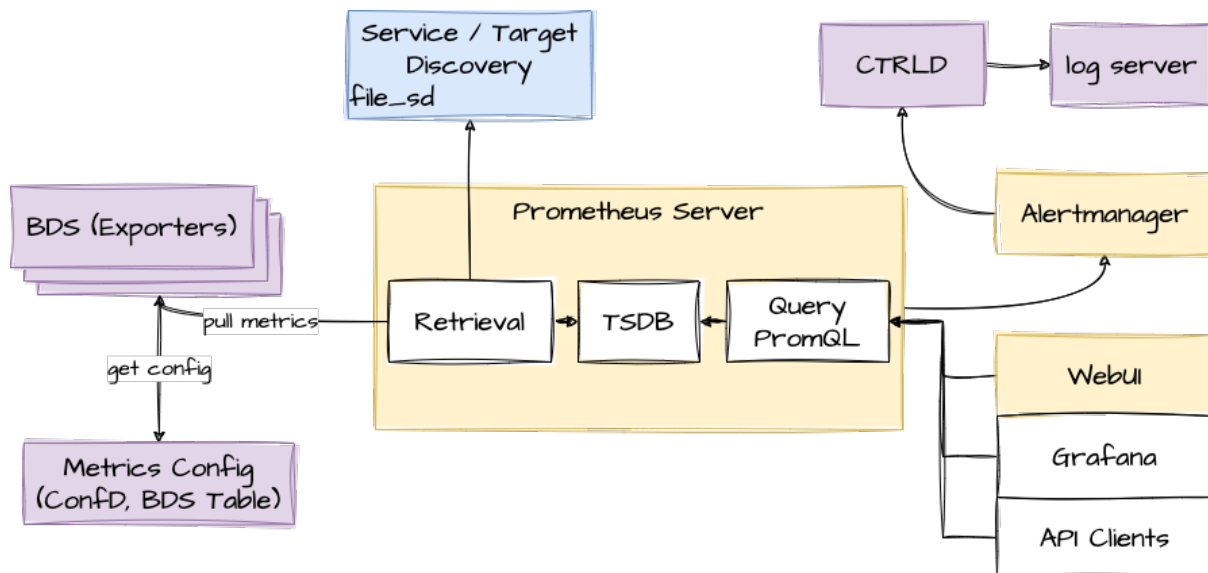
Figure 1. Prometheus in RBFS
