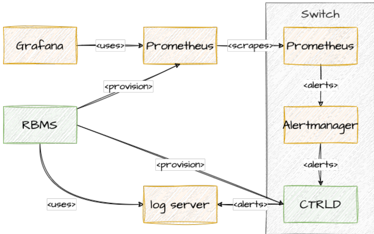
Figure 3. Federation of Prometheus, Alertmanager and graylog target
