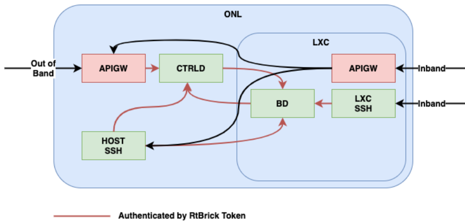
Figure 2. Internal Dataflow
